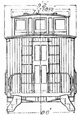
Fig. 84. End Elevation.
